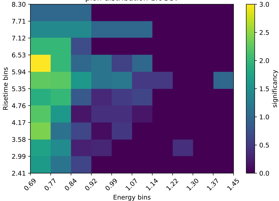
pion distribution 1.0GeV
